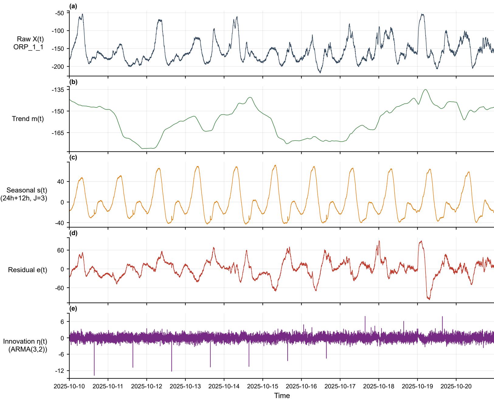
Multi-scale decomposition — ORP_1_1 (anaerobic, min) [2025-10-10~2025-10-20]
